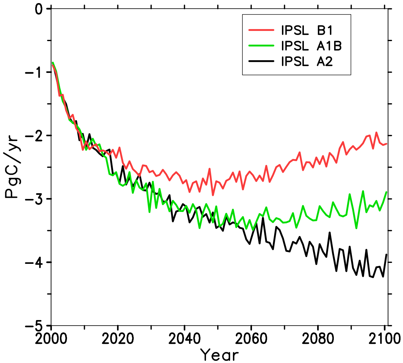
Total Flux of Carbon out of the Global Ocean
