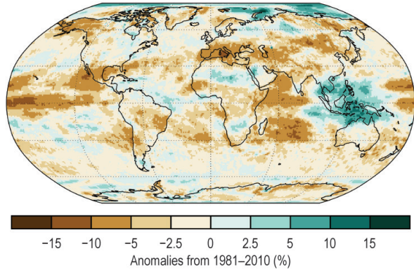
(r) Total Column Water Vapor
