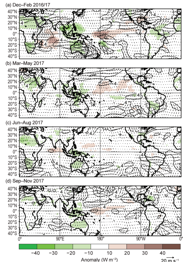
FIG. 4.5. Anomalous 200-hPa wind vectors and speed (contour interval is 4 \text{ m s}^{-1} ) and anomalous OLR (shaded, \text{W m}^{-2} ) during (a) DJF 2016/17, (b) MAM 2017, (c) JJA 2017, and (d) SON 2017. Reference wind vector is below right of color bar. Anomalies are departures from the 1981–2010 period monthly means.
