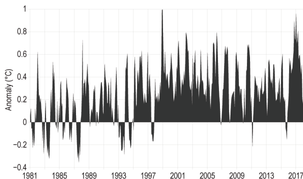
FIG. 7.51. Monthly average surface air temperature anomalies (°C, 1981–2010 base period) for the entire southwest Pacific area (25°–10°S and 156°–226°E) from 1981–2017. (Source: NOAA NCEP CPC CAMS.)
