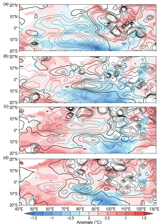
FIG. 4.41. SST (°C; colors) and precipitation (contoured at: 0, ±0.5, ±1, ±2, ±3, ±4, and ±5 mm day -1 ). Solid/dashed lines denote positive/negative values, and thick solid lines indicate the zero contour) anomalies during (a) Dec 2016–Feb 2017, (b) Mar–May 2017, (c) Jun–Aug 2017, and (d) Sep–Nov 2017. Anomalies were calculated relative to 1982–2017. [Sources: NOAA OISST (Reynolds et al. 2002) and monthly GPCP precipitation analysis (available at http://precip.gsfc.nasa.gov/ ).]
