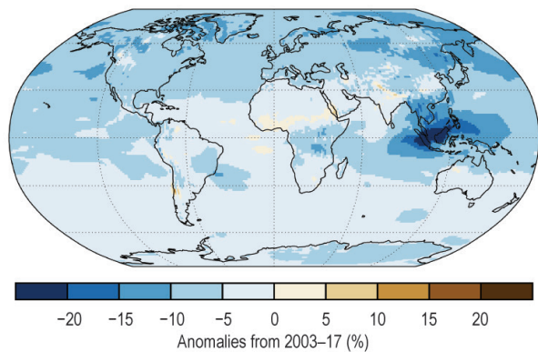
(ag) Carbon Monoxide
