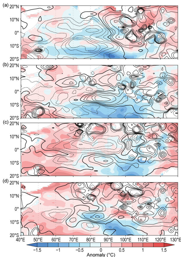
FIG. 4.41. SST ( ^{\circ}\text{C} ; colors) and precipitation (contoured at: 0, \pm 0.5 , \pm 1 , \pm 2 , \pm 3 , \pm 4 , and \pm 5 \text{mm day}^{-1} ). Solid/dashed lines denote positive/negative values, and thick solid lines indicate the zero contour) anomalies during (a) Dec 2016–Feb 2017, (b) Mar–May 2017, (c) Jun–Aug 2017, and (d) Sep–Nov 2017. Anomalies were calculated relative to 1982–2017. [Sources: NOAA OISST (Reynolds et al. 2002) and monthly GPCP precipitation analysis (available at http://precip.gsfc.nasa.gov/ ).]
