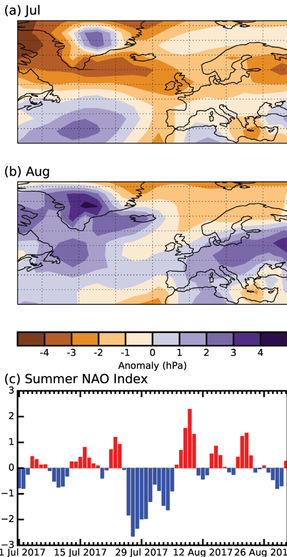
FIG. 2.37. MSLP anomalies (hPa; 1961–90 base period) in (a) Jul and (b) Aug 2017 over the extratropical North Atlantic and Europe. (c) Daily SNAO index for Jul and Aug 2017, calculated from eigenvectors of the daily SNAO.
