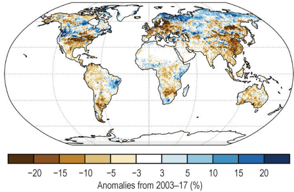
(ac) Land Surface Albedo in the Visible
