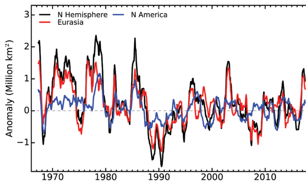
FIG. 2.14. Twelve-month running anomalies of monthly snow cover extent ( \times 10^6 km 2 ) over NH lands as a whole (black), Eurasia (red) and North America (blue) plotted on the 7th month using values from Nov 1966 to Dec 2017. Anomalies are calculated from NOAA snow maps. Mean hemispheric snow extent is 25.1 million km 2 for the full period of record. Monthly means for the period of record are used for 9 missing months between 1968 and 1971 in order to create a continuous series of running means. Missing months fall between Jun and Oct, no winter months are missing.
