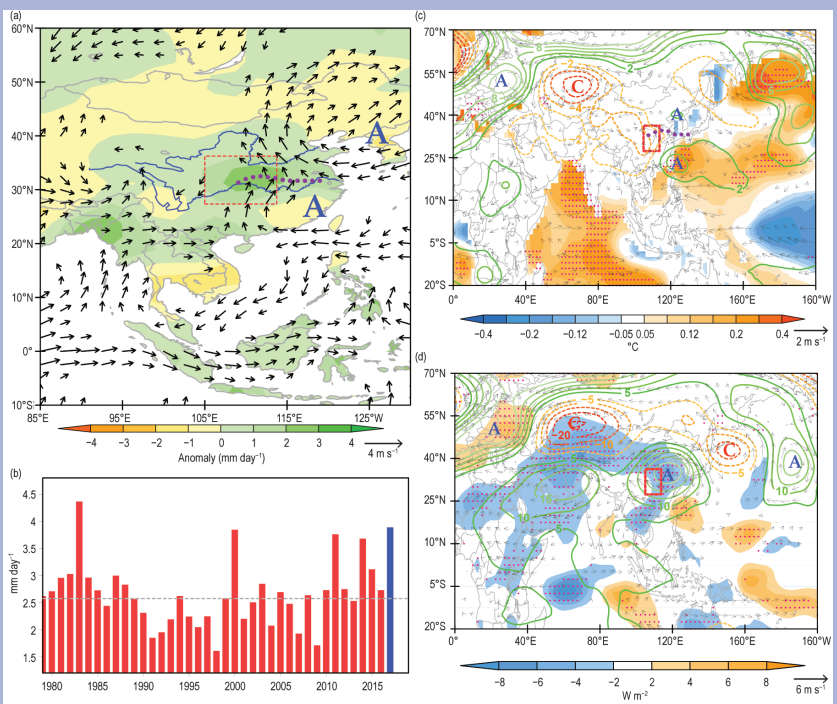
FIG. SB7.4. (a) Precipitation (shading; \text{mm day}^{-1} ) and 850-hPa wind (vector; \text{m s}^{-1} ) anomalies in Sep and Oct 2017. Only winds with speeds >1 \text{ m s}^{-1} are shown. (b) Year-to-year time series of the WCAR (red bars; \text{mm day}^{-1} ). 2017 is blue bar. Gray dashed line is the 1981–2010 climatological mean. (c) Wind (vectors; \text{m s}^{-1} ), geopotential height (contours; gpm) at 850-hPa, and SST ( ^{\circ}\text{C} ) fields regressed onto the WCAR index. (d) as in (c) but for 200-hPa wind, geopotential height, and OLR ( \text{W m}^{-2} ) fields. Only winds significant at the 95% confidence level are shown, and the SST and OLR significant at 95% confidence level are marked by red dots. “A and C” denotes the anticyclonic (cyclonic) anomaly. Red box indicates the key region of WCAR, dashed purple line marks the horizontal trough.
