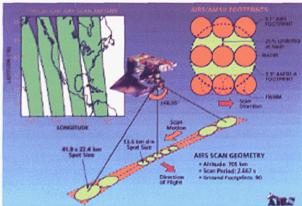
AIRS/AMSU Scan Patterns
