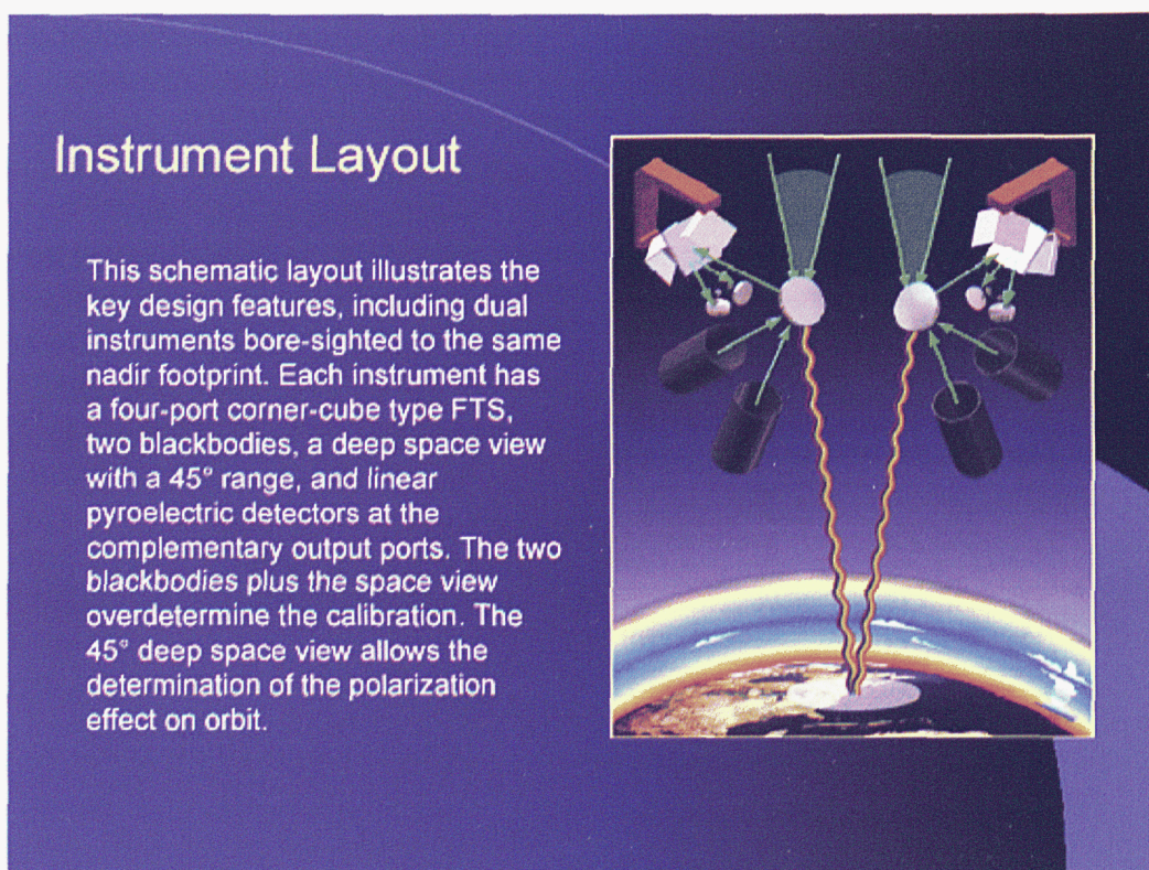
Proposed dual interferometer for very accurate spectrally resolved longwave radiation observations (Goody, Invited Workshop Presentation).
