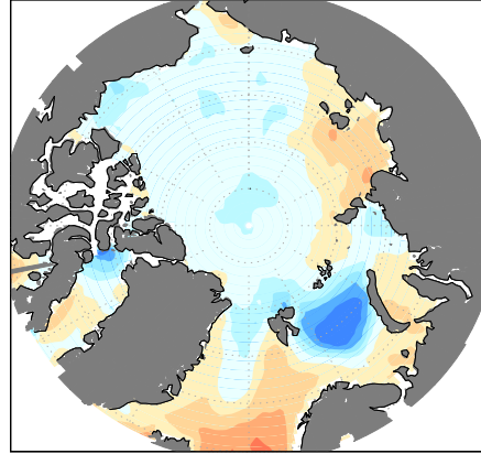
SST: Anom Summer JAS 2003 Ref:1978–2007 [°C]
