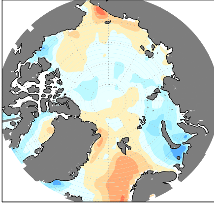
SST: Anom Summer JAS 2002 Ref:1978–2007 [°C]
