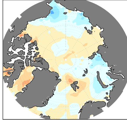
SST: Anom Summer JAS 2006 Ref:1978–2007 [°C]
