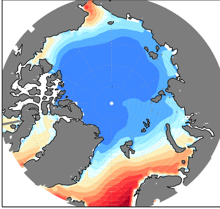
SST: Mean Summer JAS 1978–2007 [°C]
