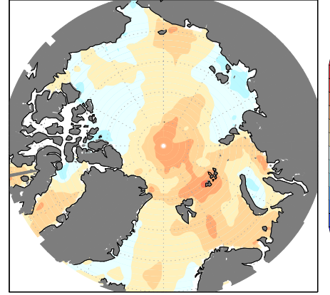
SST: Anom Summer JAS 2001 Ref:1978–2007 [°C]
