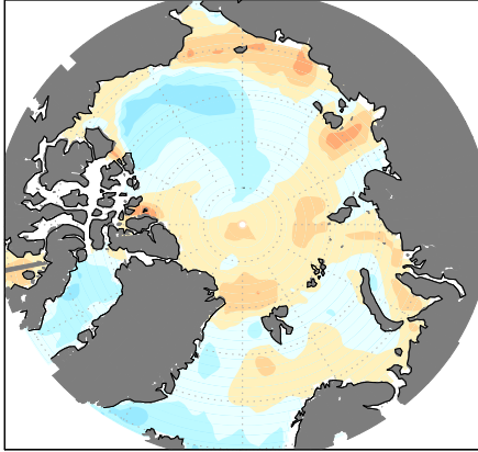
SST: Anom Summer JAS 2005 Ref:1978–2007 [°C]
