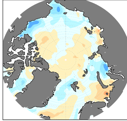
SST: Anom Summer JAS 2000 Ref:1978–2007 [°C]
