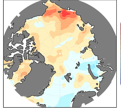
SST: Anom Summer JAS 2007 Ref:1978–2007 [°C]
