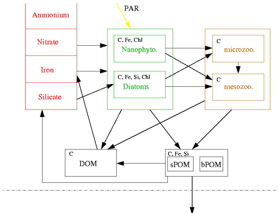
Figure 1. Architecture of PISCES. This figure only shows the ecosystem model omitting thus oxygen and the carbonate system. The elements which are explicitly modeled are indicated in the left corner of each box.
