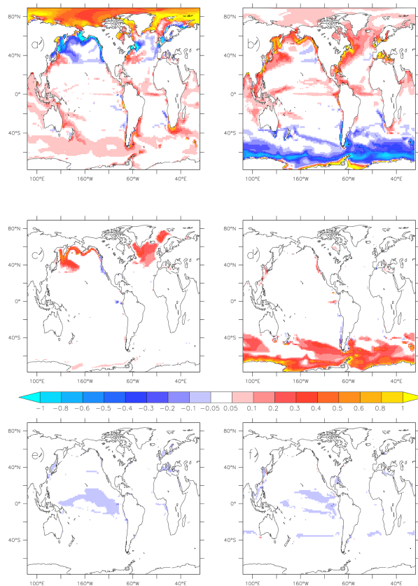
Figure 18. Surface seasonal mean Chlorophyll anomaly ( \text{mg chl a m}^{-3} ) relative to the standard simulation in April–May–June (left column) and November–December–January (right column). Panels (a) and (b) correspond to the LIGHT test; panels (c) and (d) show to the SIZE test; panels (e) and (f) display the FOOD test.
