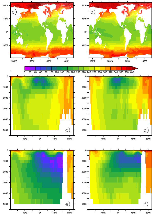
Figure 12. Annual mean O_2 concentrations in \mu\text{mol L}^{-1} . Observations are from the World Ocean Atlas 2009 (Garcia et al., 2010). Panels are the same as on Fig. 10.
