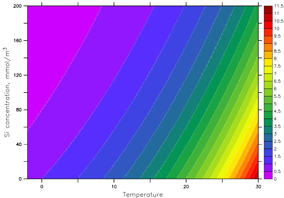
Figure 4. Dissolution rate of PSI ( \lambda_{PSi}^* ) normalized to its value at 0°C with no silicate. Temperature is in °C.
