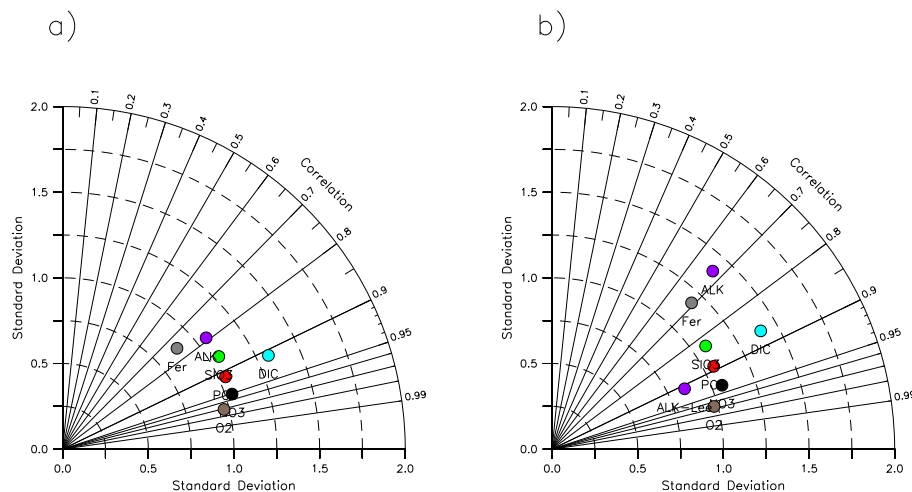
Figure 17. Taylor diagrams of model-observation comparisons for nutrients using monthly mean fields. The data are identical to those used in previous plots. Panel (a) corresponds to the global ocean. Panel (b) shows the comparison restricted to the top 100 m of the ocean. Black dot corresponds to \text{NO}_3 , brown dot to \text{O}_2 , red dot to \text{PO}_4 , green dot to \text{SiO}_3 , light blue dot to DIC, purple dot to Alkalinity and gray dot to iron. The additional purple dot labeled as Alk-Lee uses the database constructed by Lee et al. (2006) to compare with the model.
