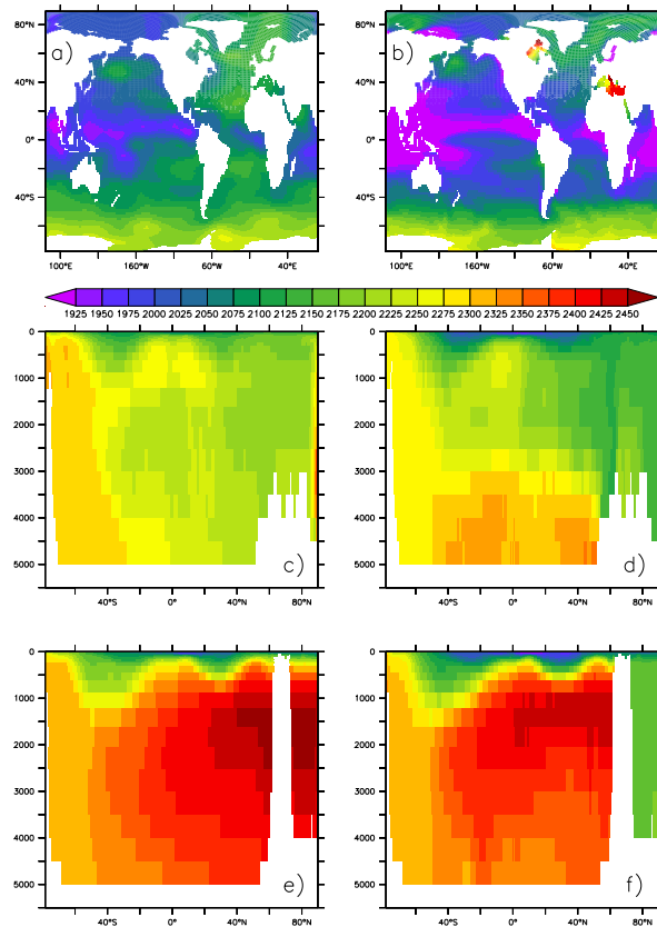
Figure 13. Annual mean DIC concentrations in \mu\text{mol L}^{-1} . Observations are from GLODAP. Panels are the same as on Fig. 10.
