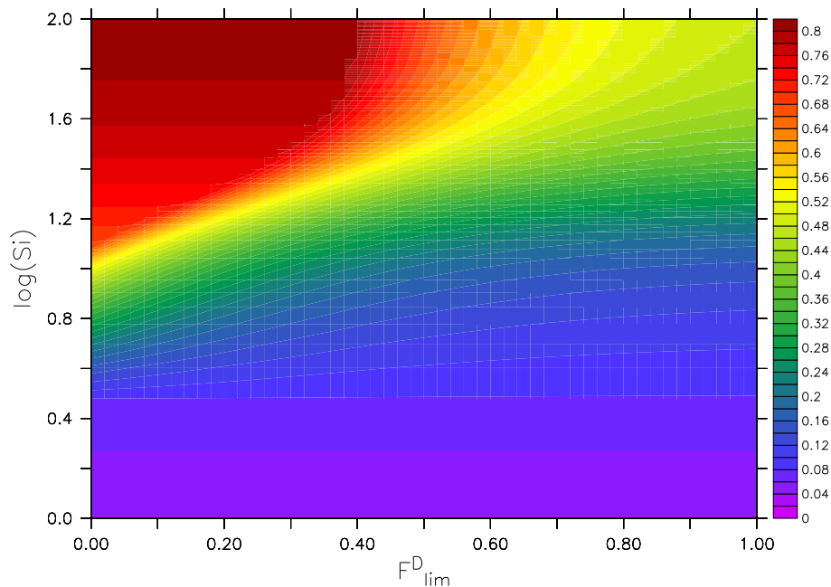
Figure 3. \theta_{opt}^{Si,D} as a function of Si concentration and F_{lim,1}^{D,Si} . The vertical axis corresponds to \log(\text{Si}) .
