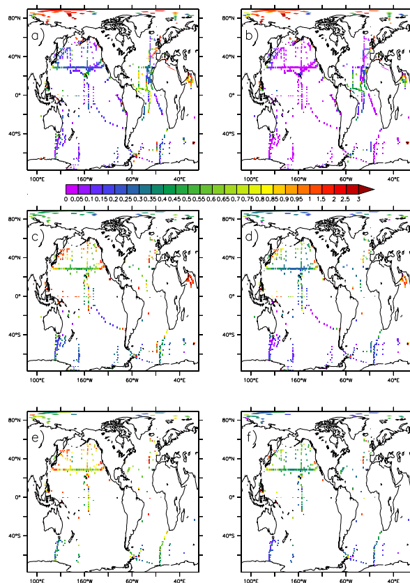
Figure 9. Spatial distribution of annual mean iron concentrations (in \text{nmol L}^{-1} ) as observed (left column) and as simulated by PISCES (right column). On panels (a) and (b), iron has been averaged over the top 50 m of the ocean. On panels (b) and (c), iron has been averaged over 200–1000 m. The bottom two panels display the iron distributions average over the depth range 1000–5000 m. Model values have been sampled at the same location and month as the data.
