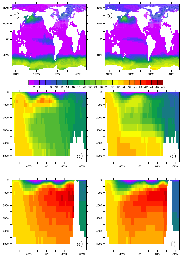
Figure 10. Annual mean \text{NO}_3 concentrations in \mu\text{mol NL}^{-1} . Observations are from the World Ocean Atlas 2009 (Garcia et al., 2010). (a) Observed surface. (b) Model run surface. (c) Observed transect zonally averaged over the Atlantic. (d) Same as (c) but for the model. (e) Observed transect zonally averaged over the Pacific. (f) Same as (e) but for the model.
