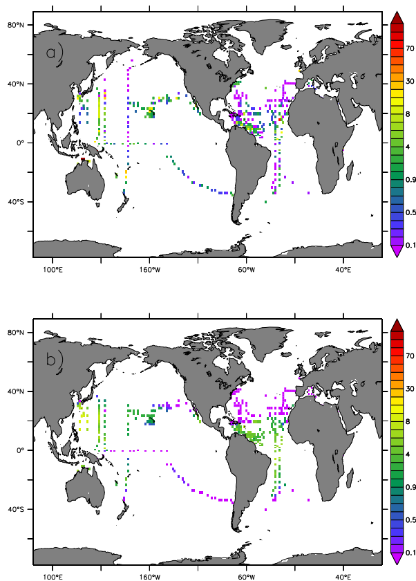
Figure 6. Annual-mean depth averaged N_2 fixation rates in \mu\text{mol N m}^{-2} \text{d}^{-1} . (a) Database from the MAREMIP project (Luo et al., 2013); (b) model predictions.
