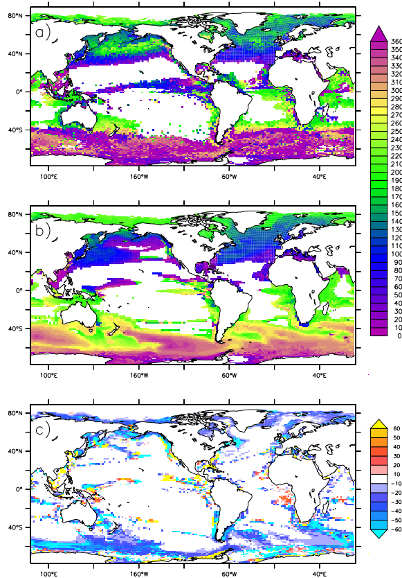
Figure 19. Day of the year at which sea surface chlorophyll is maximum. Panel (a) corresponds to the observations; panel (b) displays the standard simulation. Panel (c) shows the difference between the LIGHT and the standard experiments. Only the regions where the amplitude of the seasonal cycle exceeds 0.1 \text{ mg chl a m}^{-3} are shown.
