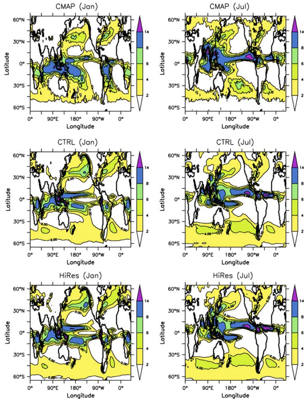
Fig. 9 January ( left ) and July ( right ) precipitation (in \text{mm day}^{-1} ) for CMAP (Xie and Arkin 1997) data ( top ), CTRL ( middle ) and HiRes ( bottom ). See Table 4 for global averages and Fig. 5 for statistics
