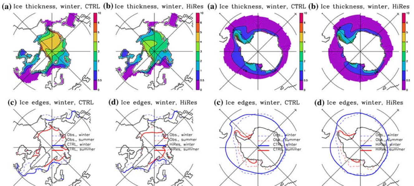
Fig. 14 Winter sea ice thickness for the model ( top ), and winter and summer ice edges ( bottom ) for model and data (Gloersen and Campbell 1991). See Table 4 for global averages and Fig. 5 for statistics
